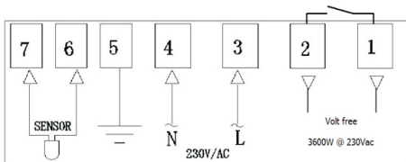
Voltage-Free System
