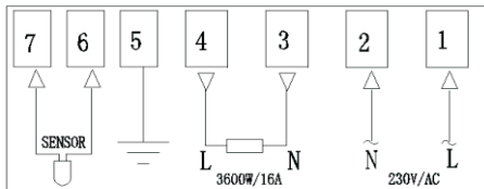
Electric Heating System
